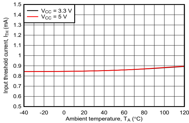
ISOM871x Figure 7-1. Input Threshold Current vs Ambient Temperature
