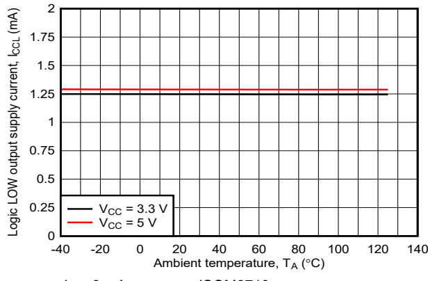
Figure 7-15. Logic LOW Output Supply Current vs Ambient Temperature
