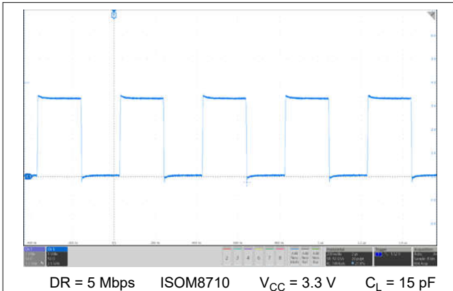
Figure 10-2. Typical Output Waveform at I_F = 2\text{ mA}
