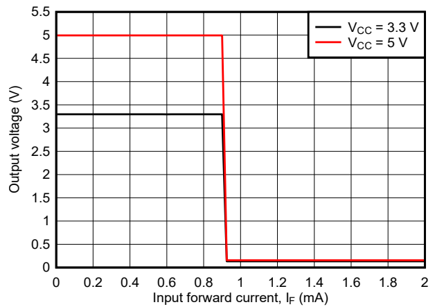
ISOM8711 T_A = 25^\circ\text{C} Figure 7-4. Output Voltage vs Input Forward Current
