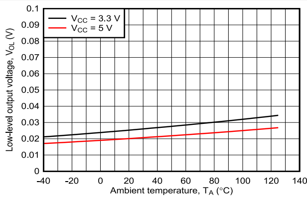
ISOM8710 I_F = 6\text{ mA} I_{OL} = 2\text{ mA} Figure 7-5. Low-Level Output Voltage vs Ambient Temperature
