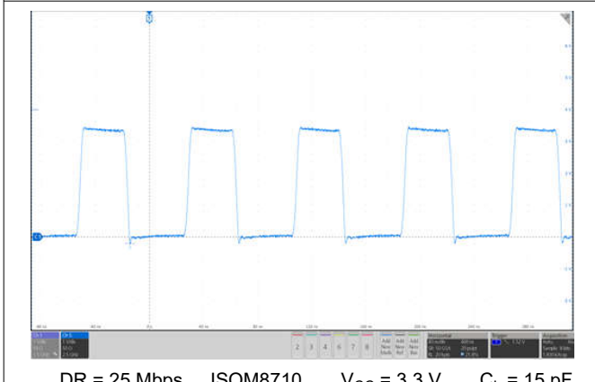
Figure 10-6. Typical Output Waveform at I_F = 6\text{ mA}
