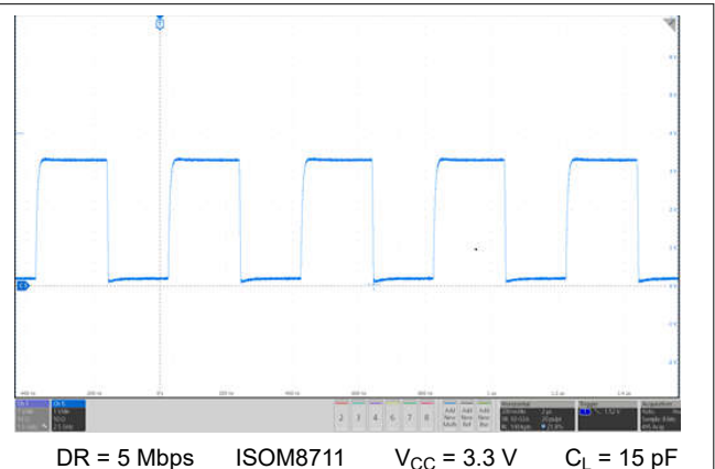
Figure 10-3. Typical Output Waveform at I_F = 2\text{ mA}
