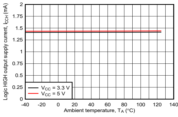
Figure 7-17. Logic HIGH Output Supply Current vs Ambient Temperature
