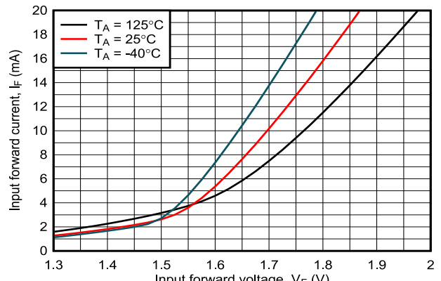
ISOM871x Figure 7-2. Input Forward Current vs Input Forward Voltage
