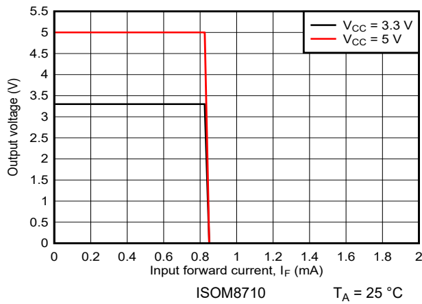
ISOM8710 T_A = 25^\circ\text{C} Figure 7-3. Output Voltage vs Input Forward Current
