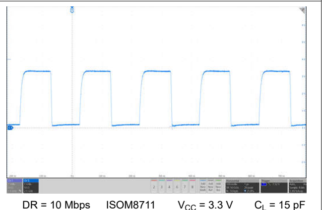
Figure 10-5. Typical Output Waveform at I_F = 3\text{ mA}
