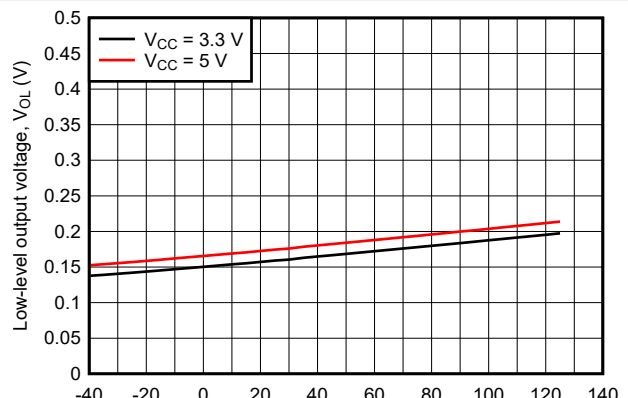
ISOM8711 I_F = 6\text{ mA} I_{OL} = 2\text{ mA} Figure 7-6. Low-Level Output Voltage vs Ambient Temperature
