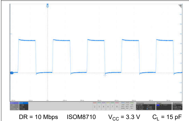
Figure 10-4. Typical Output Waveform at I_F = 3\text{ mA}
