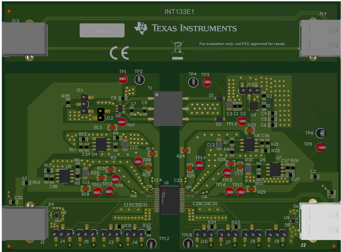
Figure 6-4. ISOUSB211DPEVM PCB 3D View
