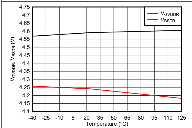
Figure 6-12. GVDD and BST UVLO Thresholds vs Temperature
