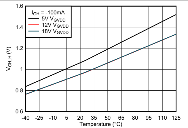
Figure 6-9. GH Output High Voltage vs Temperature
