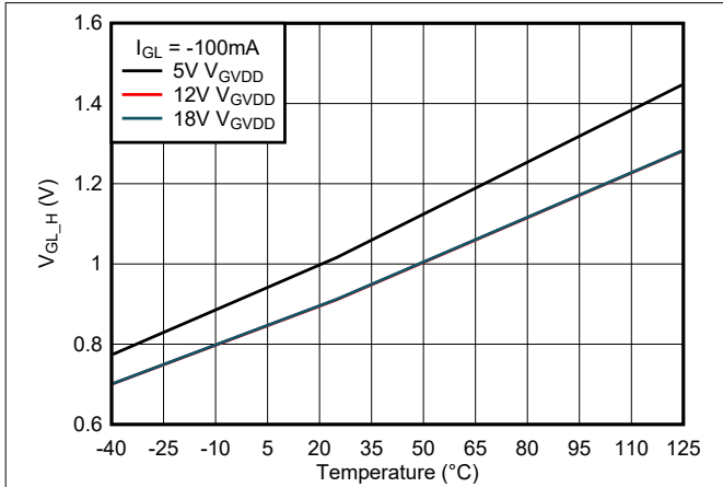
Figure 6-8. GL Output High Voltage vs Temperature
