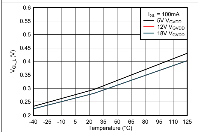
Figure 6-10. GL Output Low Voltage vs Temperature
