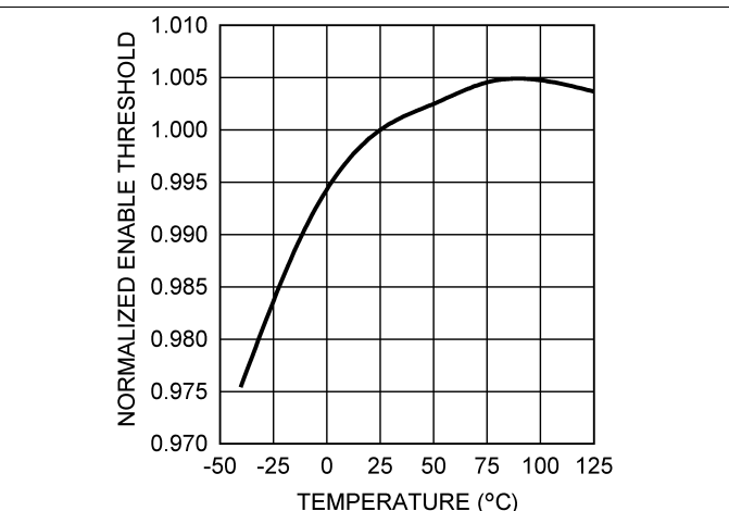
Figure 6. Normalized Enable Threshold Voltage vs Temperature
