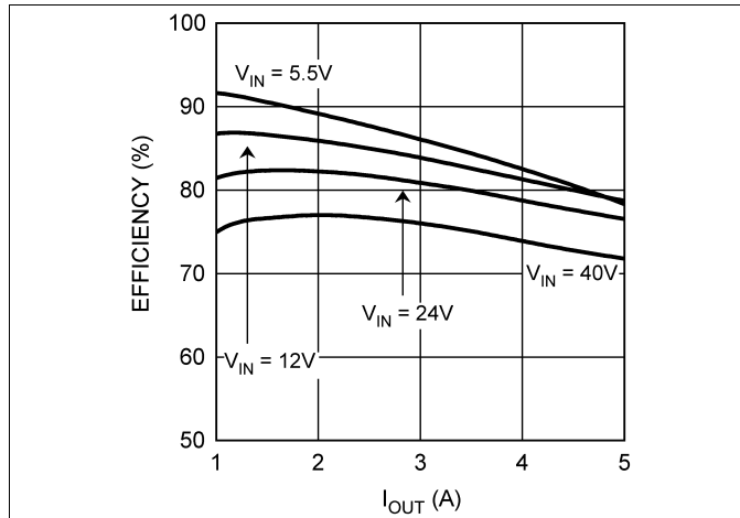
Figure 1. Efficiency vs I_{OUT} and V_{IN} , V_{OUT} = 3.3\text{ V}
