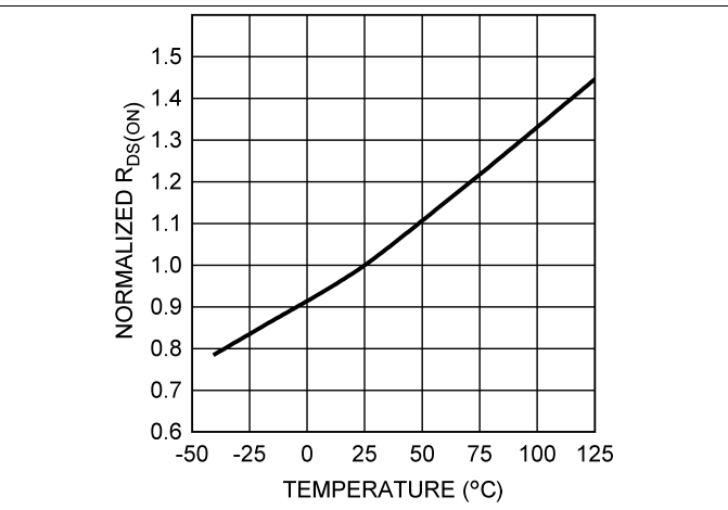
Figure 4. Normalized R_{DS(ON)} vs Temperature
