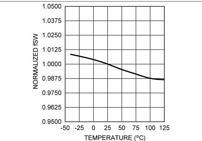
Figure 2. Normalized Switching Frequency vs Temperature
