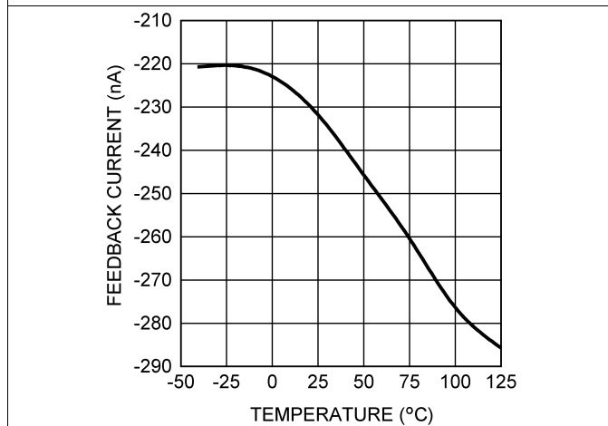
Figure 5. Feedback Bias Current vs Temperature
