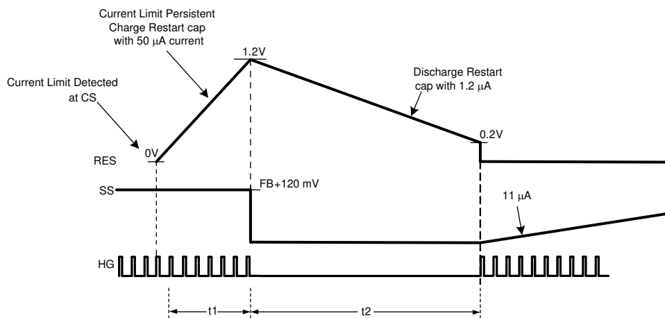
图 7-8. Current Limit Restart Timing Diagram
