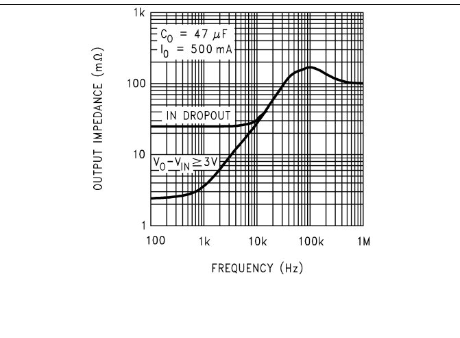
Figure 16. LM2990-12 and LM2990-15 Output Impedance
