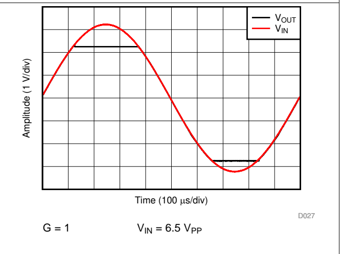
Figure 21. No Phase Reversal
