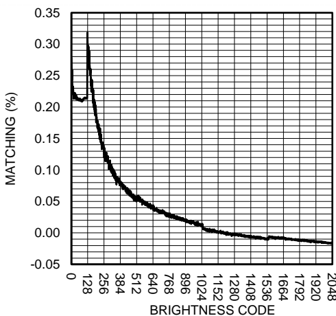
图 46. LED Matching (Linear Mapping)
