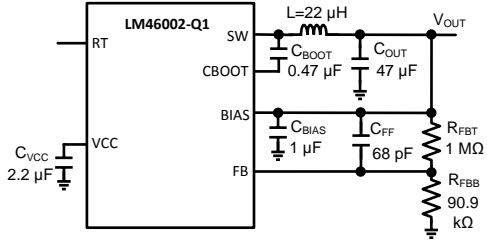
V_{OUT} = 12\text{ V} F_S = 500\text{ kHz}
