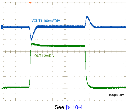
图 8-5. Load Transient Response
