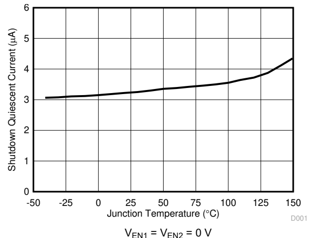
图 8-6. Shutdown Current Versus Temperature
