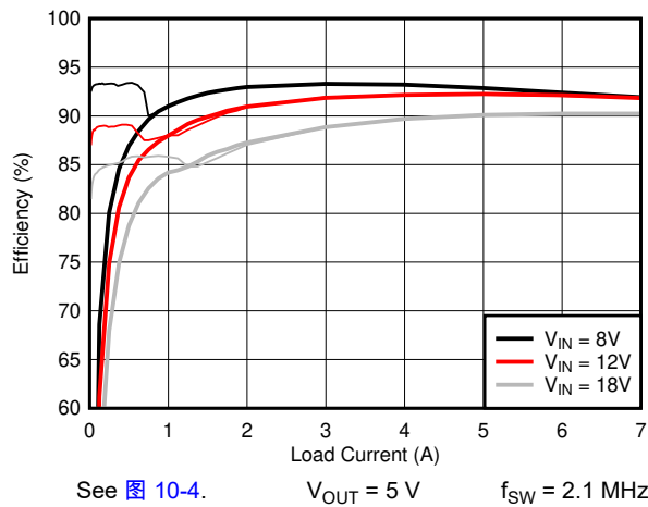
图 8-1. Efficiency Versus Load
