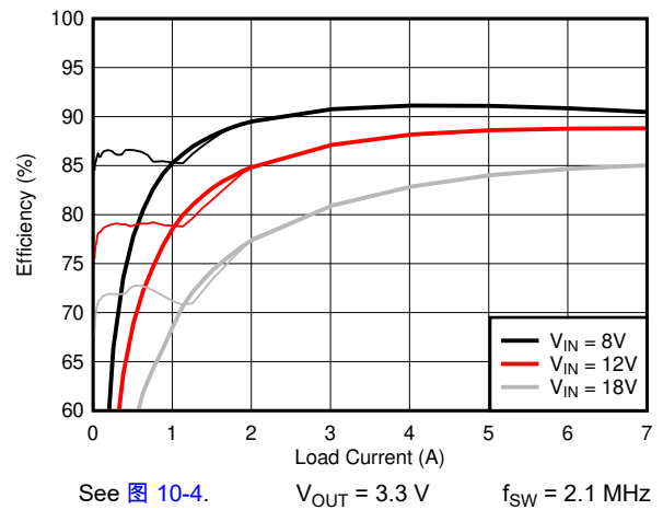
图 8-2. Efficiency Versus Load
