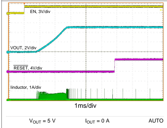
Figure 27. Start-up
