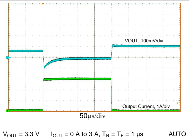
Figure 40. Load Transient
