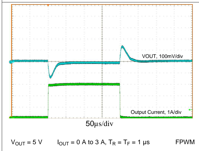
Figure 29. Load Transient
