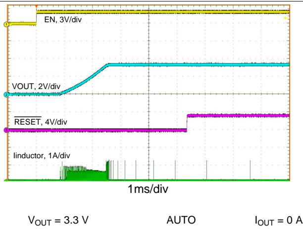
Figure 39. Start-up
