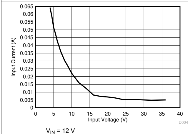
图 7-5. Short Circuit Average Input Current for LM53635-Q1
