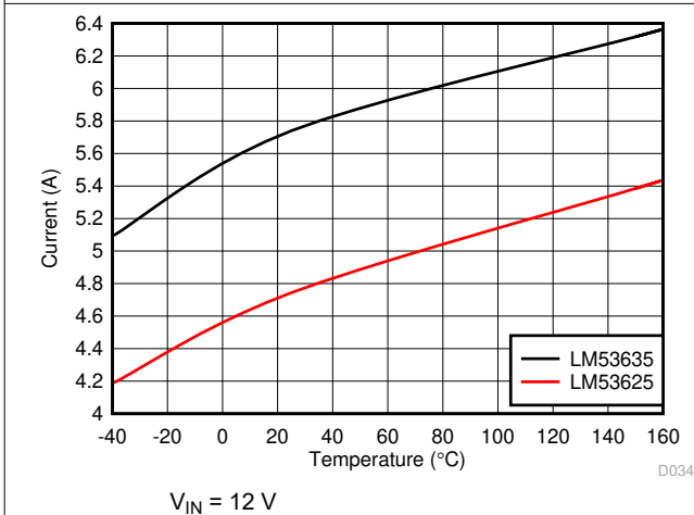
图 7-3. High Side/Peak Current Limit for LM53625/35-Q1
