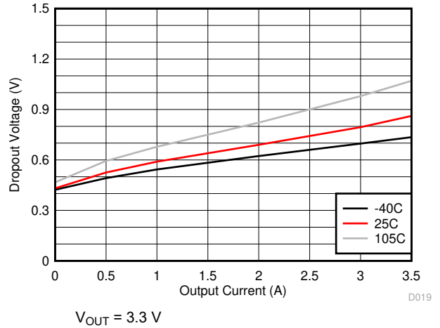
图 9-26. Dropout for \geq 1.85\text{ MHz}
