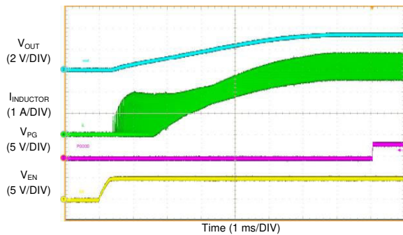
图 10-31. LM61460-Q1 Start-up with 50-mA Load
