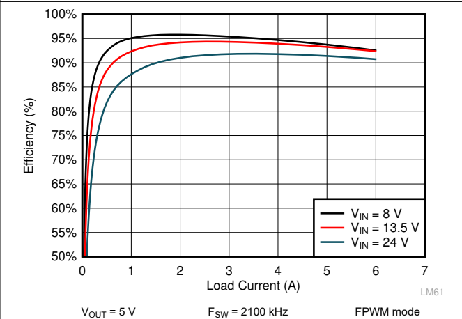
图 9-16. LM61460 Efficiency
