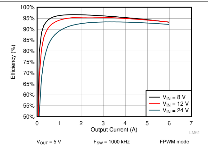
图 9-14. LM61460 Efficiency
