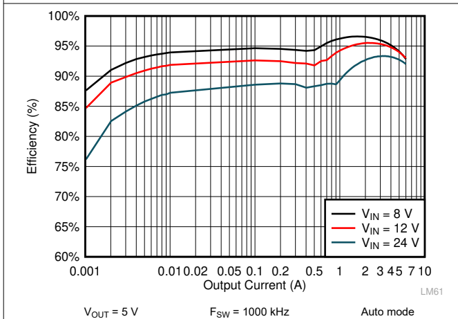
图 9-13. LM61460 Efficiency
