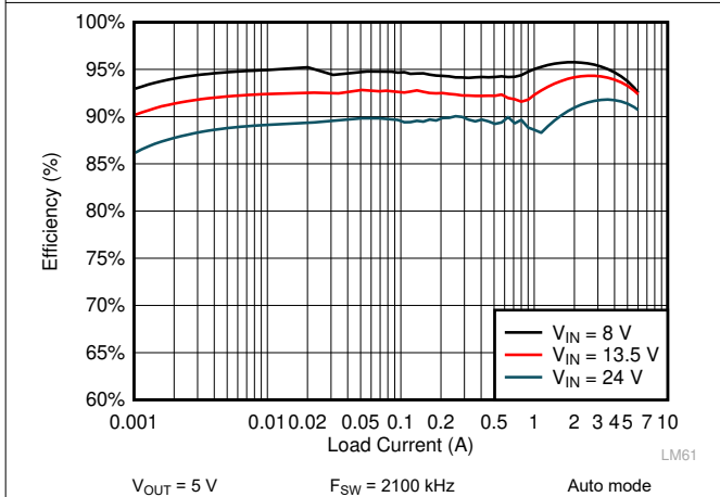
图 9-15. LM61460 Efficiency
