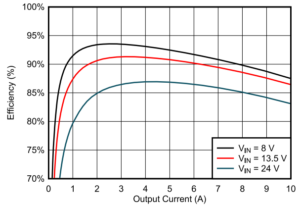
图 9-12. Efficiency
