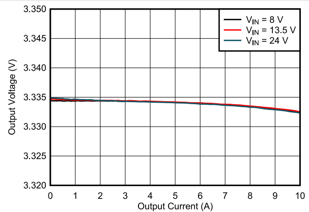
图 9-14. Load and Line Regulation
