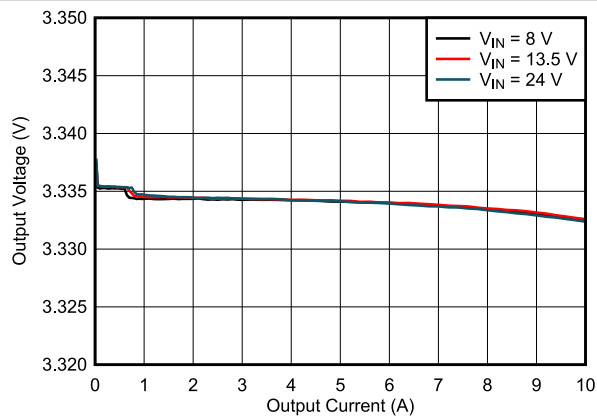
图 9-13. Load and Line Regulation
