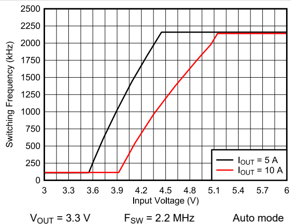
图 9-28. Frequency Dropout
