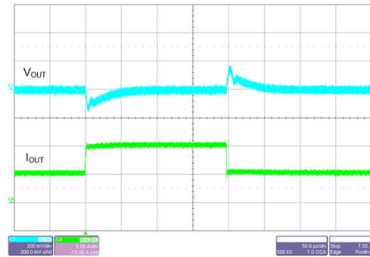
V_{OUT} = 3.3\text{ V} F_{SW} = 400\text{ kHz} Auto mode I_{OUT} = 5\text{ A to }10\text{ A to }5\text{ A} V_{IN} = 13.5\text{ V} T_R = T_F = 1\text{ }\mu\text{s}
