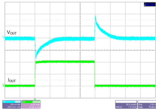
V_{OUT} = 5\text{ V} F_{SW} = 2200\text{ kHz} FPWM mode I_{OUT} = 10\text{ mA to }10\text{ A to }10\text{ mA} V_{IN} = 13.5\text{ V} T_R = T_F = 1\text{ }\mu\text{s}
