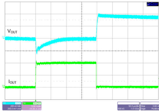
V_{OUT} = 3.3\text{ V} F_{SW} = 400\text{ kHz} Auto mode I_{OUT} = 10\text{ mA to }10\text{ A to }10\text{ mA} V_{IN} = 13.5\text{ V} T_R = T_F = 1\text{ }\mu\text{s}
