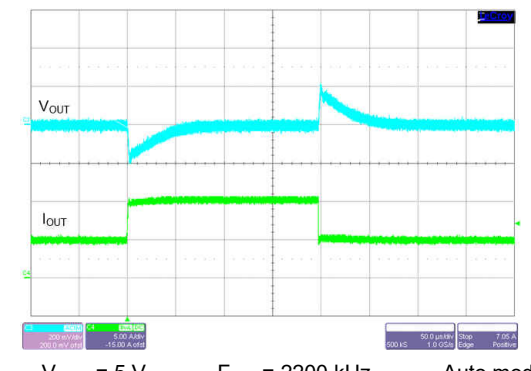
V_{OUT} = 5\text{ V} F_{SW} = 2200\text{ kHz} Auto mode I_{OUT} = 5\text{ A to }10\text{ A to }5\text{ A} V_{IN} = 13.5\text{ V} T_R = T_F = 1\text{ }\mu\text{s}
