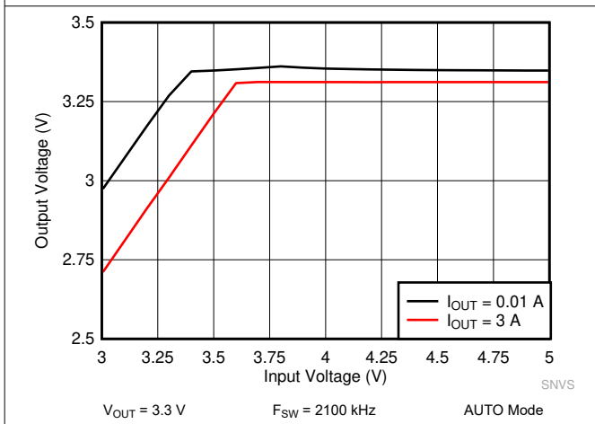
图 10-13. LM62440-Q1 Dropout Curve
