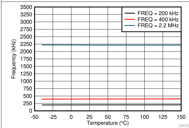
图 8-5. Switching Frequency Set by SYNC
