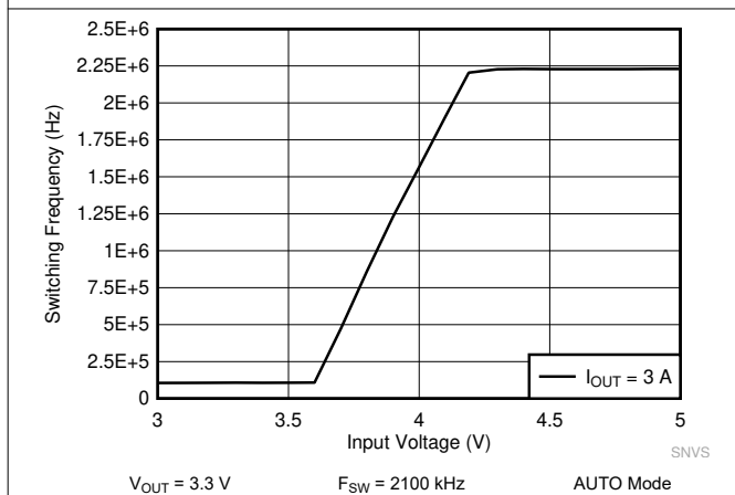
图 10-15. LM62440-Q1 Frequency Dropout Curve
