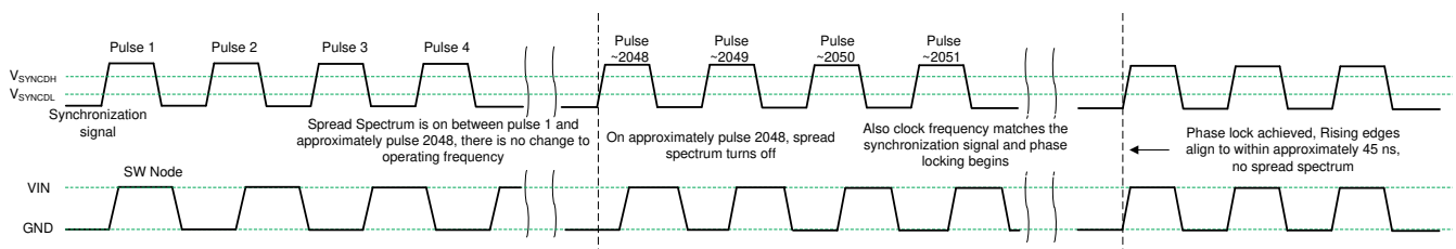
图 9-12. Synchronization Process
