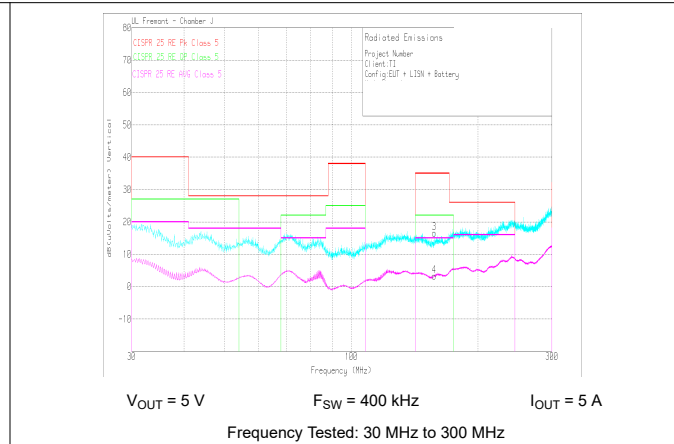
图 10-30. Radiated EMI Bicon Horizontal versus CISPR25 Limits
