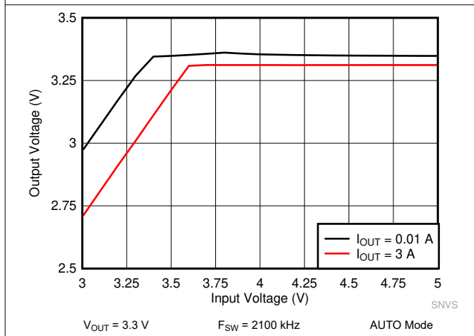
图 10-13. LM62440-Q1 Dropout Curve
