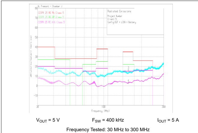
图 10-29. Radiated EMI Bicon Vertical versus CISPR25 Limits
