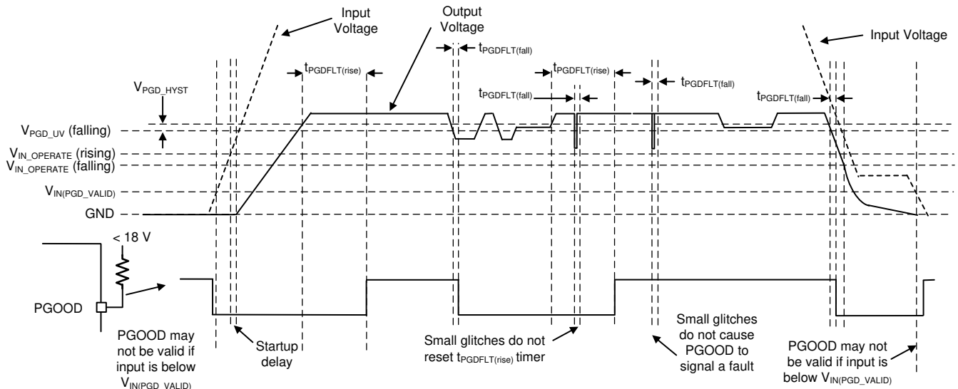
图 9-13. PGOOD Timing Diagram (Excludes OV Events)
