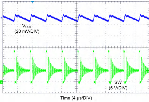
图 10-17. LM62440-Q1 Switching Waveform and V_{OUT} Ripple
