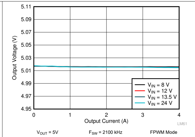
图 10-12. LM62440-Q1 Load and Line Regulation
