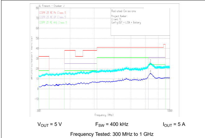
图 10-31. Radiated EMI Log Vertical versus CISPR25 Limits
