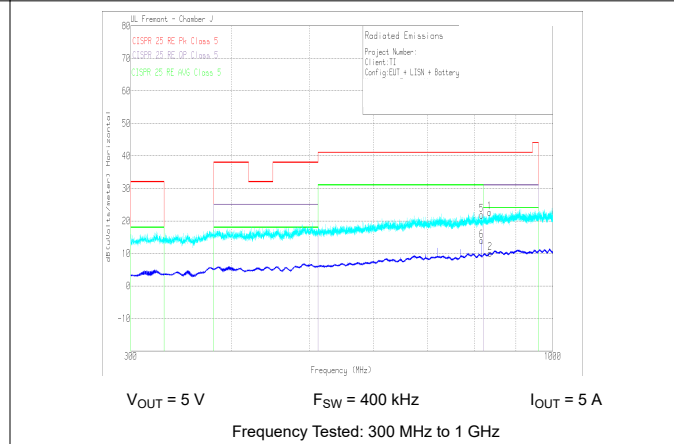
图 10-32. Radiated EMI Log Horizontal versus CISPR25 Limits
