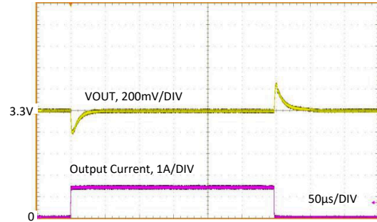
LM63615 V_{OUT} = 3.3V f_{SW} = 2100\text{ kHz} 0A 至 1.5A, 2µs FPWM
