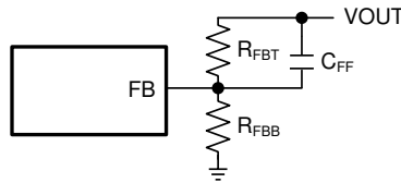
图 8-14. Feedforward Capacitor for Loop Compensation
