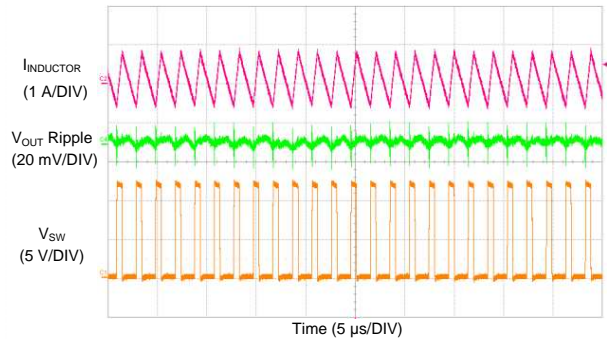
图 58. LM73606 Switching Waveform and V_{OUT} Ripple
