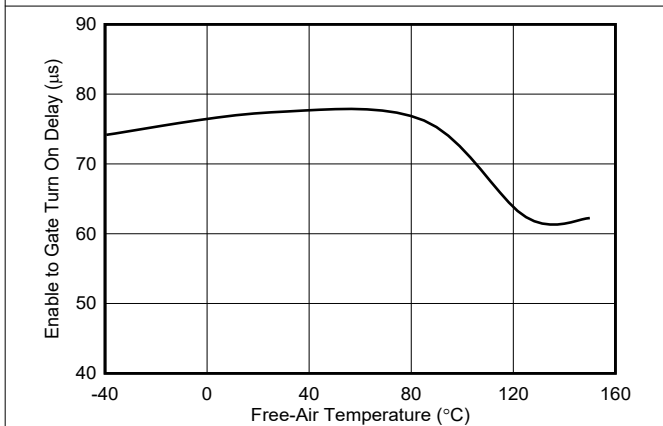
图 6-11. Enable to Gate Delay vs Temperature
