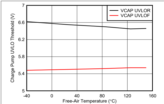
图 6-13. Charge Pump UVLO Threshold vs Temperature
