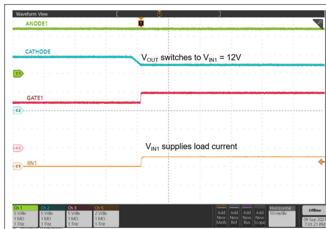
图 9-15. ORing V_{IN2} to V_{IN1} Switch Over
