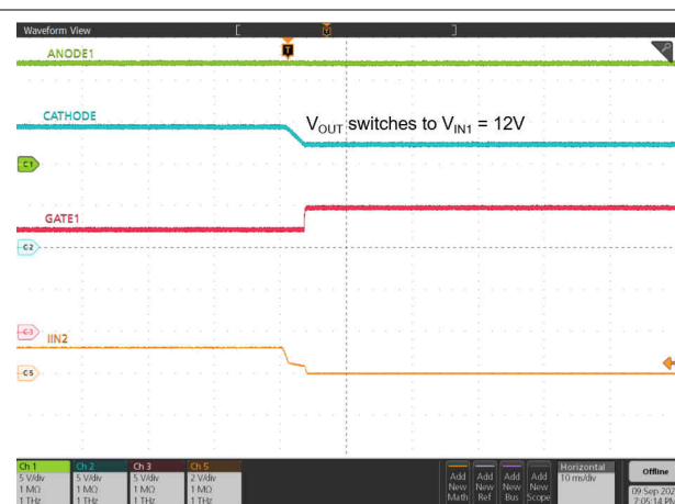
图 9-16. ORing V_{IN2} to V_{IN1} Switch Over
