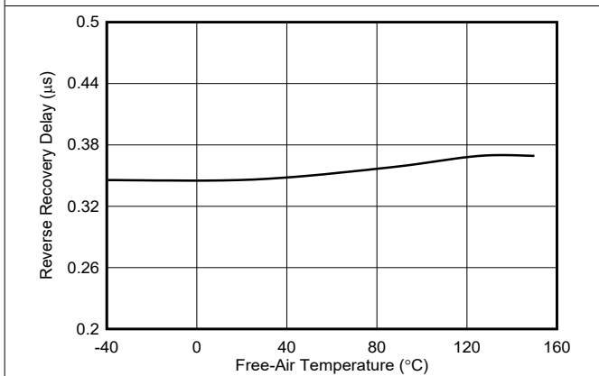
图 6-9. Reverse Current Blocking Delay vs Temperature
