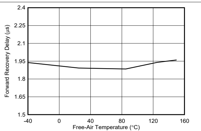
图 6-10. Forward Recovery Delay vs Temperature
