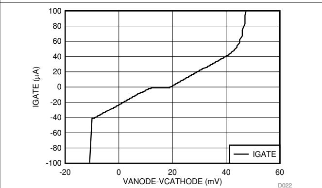
图 6-16. Gate Current vs Forward Voltage Drop
