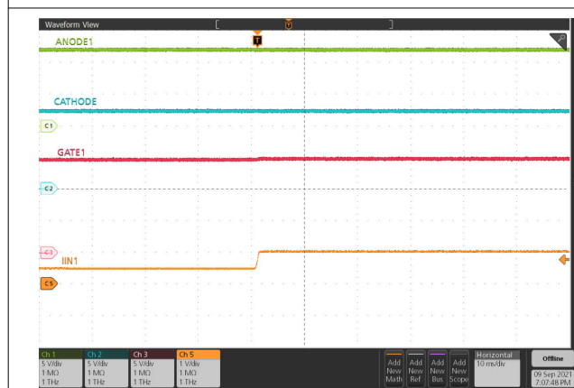
图 9-15. ORing V_{IN2} to V_{IN1} Switch Over
