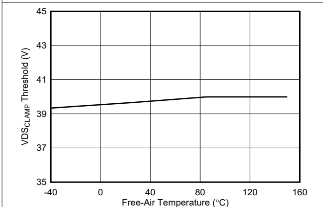
图 6-15. V_{DSCLAMP} Threshold vs Temperature
