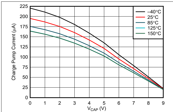
图 6-7. Charge Pump V-I Characteristics at V_{ANODE} = 3.2\text{ V}
