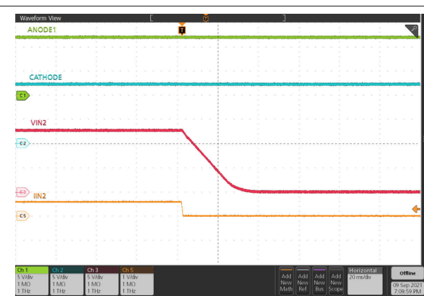
图 9-16. ORing V_{IN2} to V_{IN1} Switch Over
