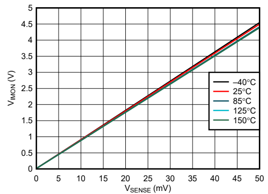
Figure 7-22. Current Monitor Output vs Sense Voltage ( R_{IMON} = 5k\Omega , R_{SET} = 50\Omega )
