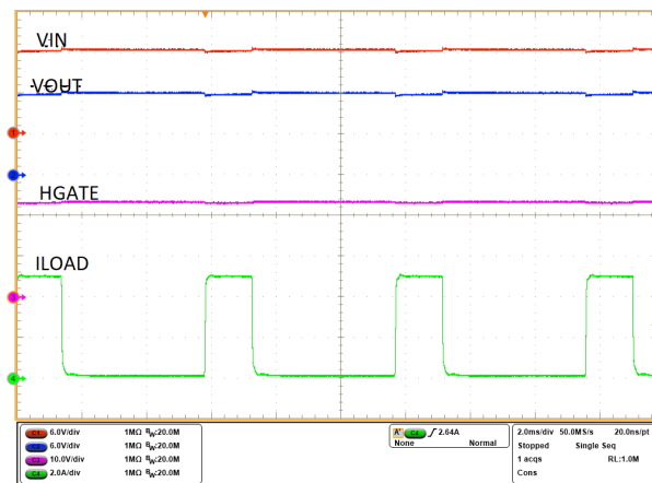
Figure 10-22. Load Transient 100 mA to 5 A
