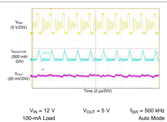
图 60. LM76003-Q1 Switching Waveform and Output Ripple
