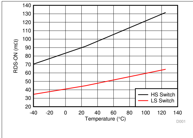
图 1. High-Side and Low-Side Switch R_{DS-ON}
