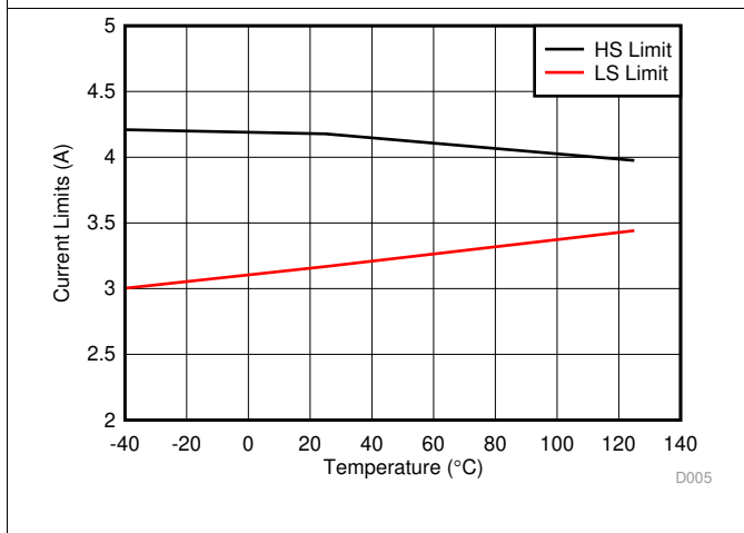
图 5. LM76002-Q1 High-Side and Low-Side Current Limits
