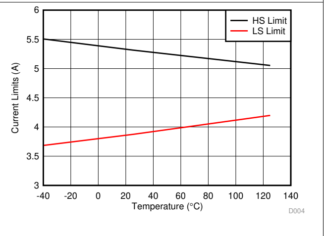
图 4. LM76003-Q1 High-Side and Low-Side Current Limits
