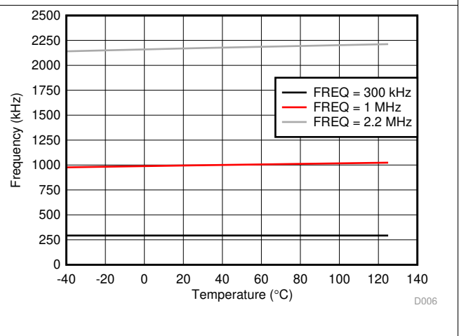
图 6. Switching Frequency Set by R_T Resistor
