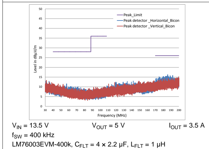
图 87. LM76003-Q1 Radiated EMI Result vs. CISPR25 Limits - Low Frequency
