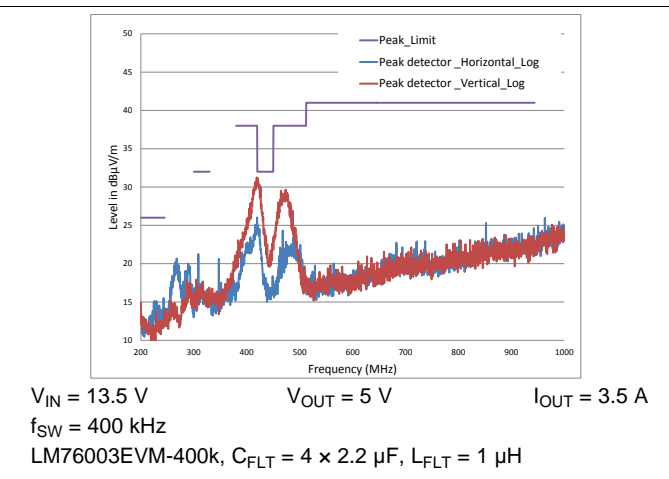
图 88. LM76003-Q1 Radiated EMI Result vs. CISPR25 Limits - High Frequency
