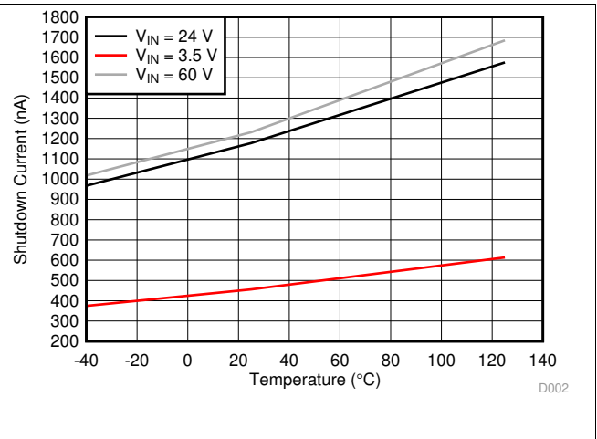
图 2. Shutdown Quiescent Current
