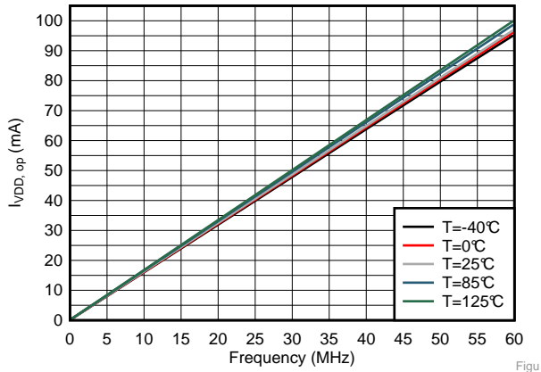
图 1. I_{VDD,op} vs Frequency With 2 \Omega Series 100 pF Load
