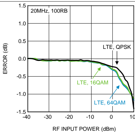
Figure 23. LTE Variation vs. RF Input Power at 900 MHz
