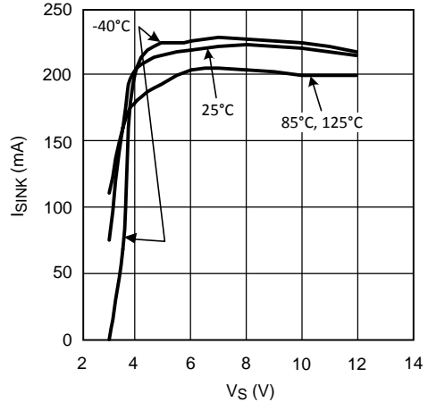
Figure 26. Short Circuit Current
