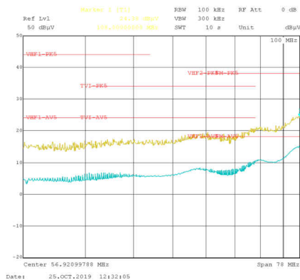
V_{OUT} = 5V F_{SW} = 400\text{ kHz} I_{OUT} = 5A 测试频率：30 MHz 至 108 MHz
