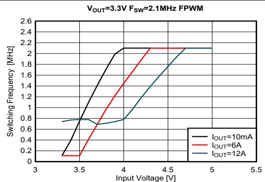
V_{OUT} = 3.3\text{ V} F_{SW} = 2.1 FPWM mode Single Output MHz
