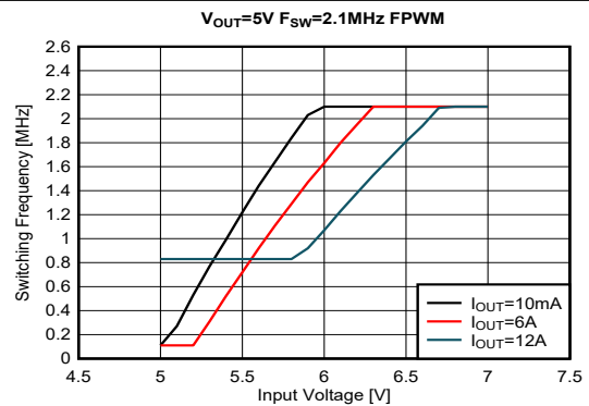
V_{OUT} = 5\text{ V} F_{SW} = 2.1 FPWM mode Single Output MHz
