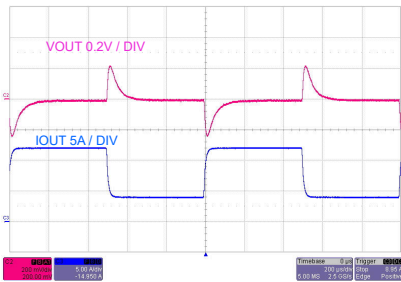
V_{OUT} = 3.3\text{ V} F_{SW} = 400\text{ kHz} FPWM mode I_{OUT} = 4\text{ A to }12\text{ A to }4\text{ A} V_{IN} = 13.5\text{ V} Single Output
