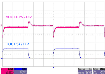
V_{OUT} = 3.3\text{ V} F_{SW} = 400\text{ kHz} Auto mode I_{OUT} = 100\text{ mA to }6\text{ A to }100\text{ mA} V_{IN} = 13.5\text{ V} Dual Output
