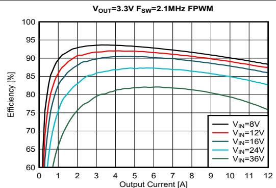
Figure 9-18. Efficiency
