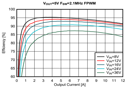
Figure 9-15. Efficiency
