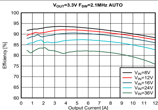
Figure 9-17. Efficiency
