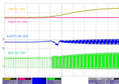
V_{OUT} = 5\text{ V} F_{SW} = 400 kHz Auto mode I_{OUT} = 3\text{ A} V_{IN} = 5\text{ to }7\text{ V} Single Output
