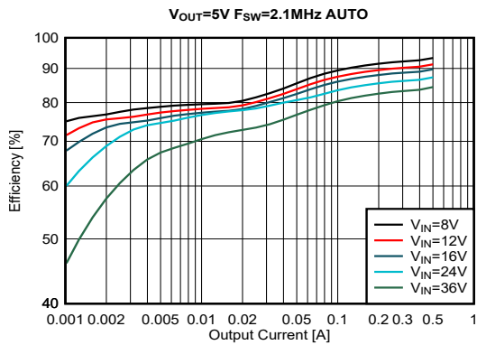
Figure 9-15. Efficiency
