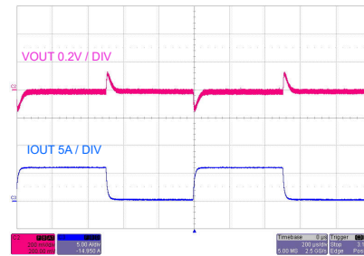
V_{OUT} = 3.3\text{ V} F_{SW} = 400\text{ kHz} FPWM mode I_{OUT} = 100\text{ mA to }6\text{ A to }100\text{ mA} V_{IN} = 13.5\text{ V} Dual Output
