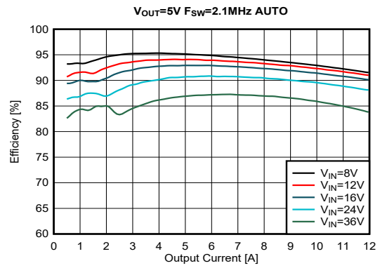
Figure 9-16. Efficiency
