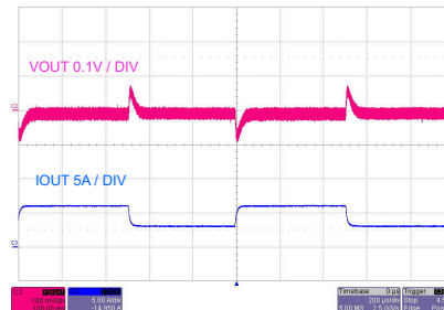
V_{OUT} = 3.3\text{ V} F_{SW} = 400\text{ kHz} FPWM mode I_{OUT} = 3\text{ A to }6\text{ A to }3\text{ A} V_{IN} = 13.5\text{ V} Dual Output
