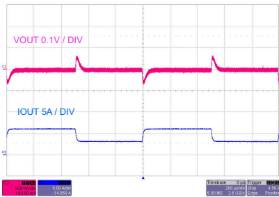
V_{OUT} = 3.3\text{ V} F_{SW} = 2.1\text{ MHz} FPWM mode I_{OUT} = 3\text{ A to }6\text{ A to }3\text{ A} V_{IN} = 13.5\text{ V} Dual Output
