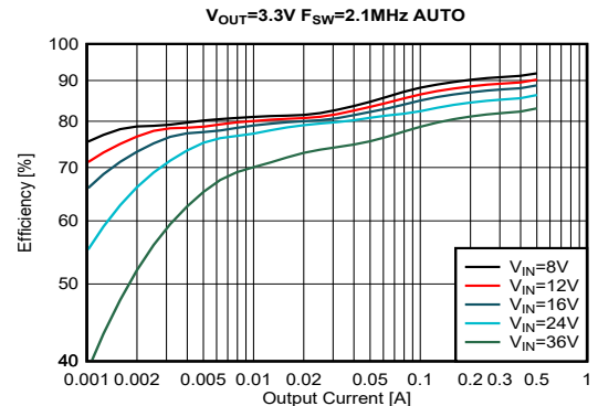
Figure 9-16. Efficiency
