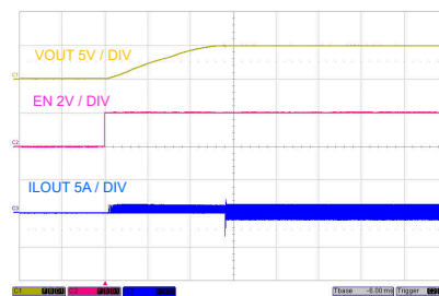
V_{OUT} = 5\text{ V} F_{SW} = 400 kHz FPWM mode I_{OUT} = 100\text{ mA} V_{IN} = 13.5\text{ V} Dual Output
