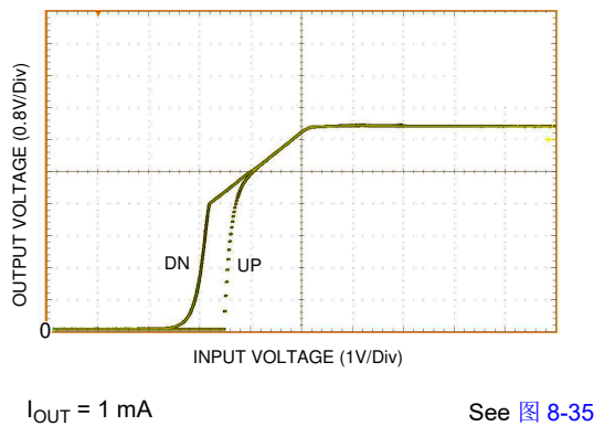
图 6-5. UVLO Thresholds
