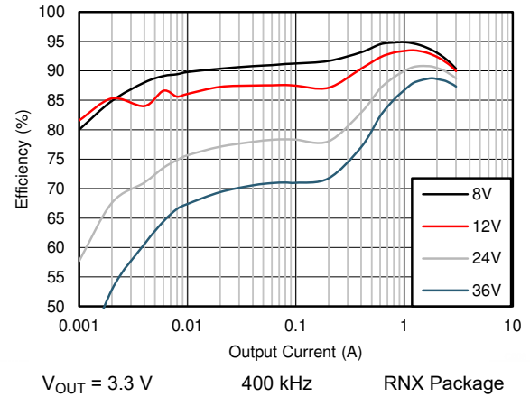
图 9-14. Efficiency
