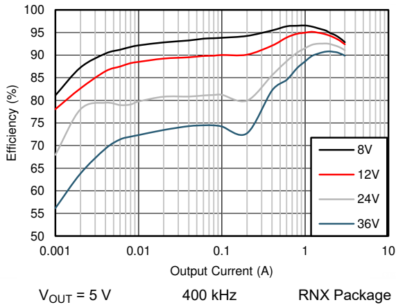
图 9-5. Efficiency
