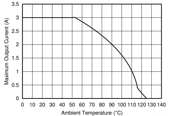
Figure 9-4. Maximum Output Current vs Ambient Temperature V_{IN} = 12\text{ V} V_{OUT} = 5\text{ V} f_{SW} = 400\text{ kHz} R_{\theta JA} = 50^{\circ}\text{C}/\text{W}
