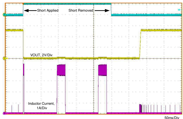
图 8-6. Short-Circuit Transient and Recovery
