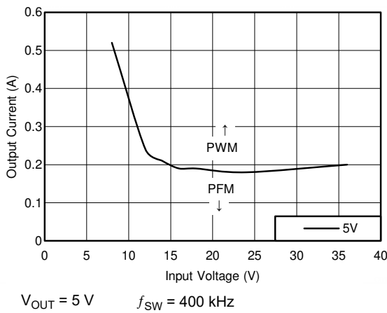
图 9-21. Mode Change Thresholds
