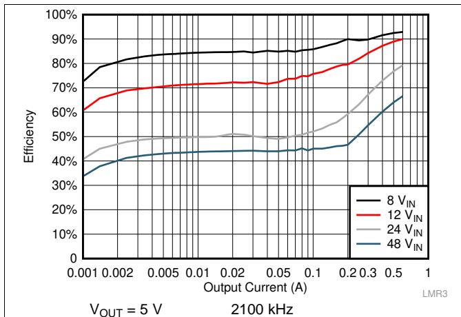
图 43. Efficiency
