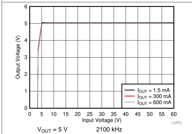
图 47. Line Regulation
