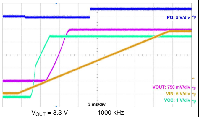
图 30. Start-Up Waveform
