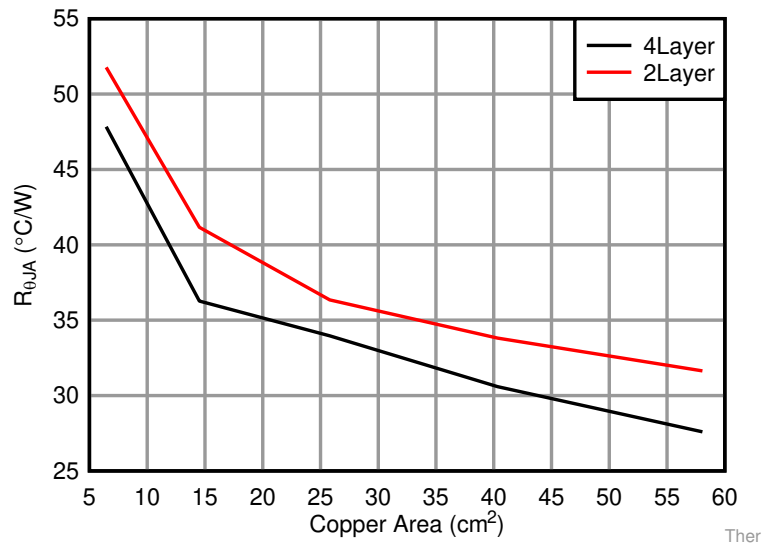
图 15. R θJA versus Copper Board Area
