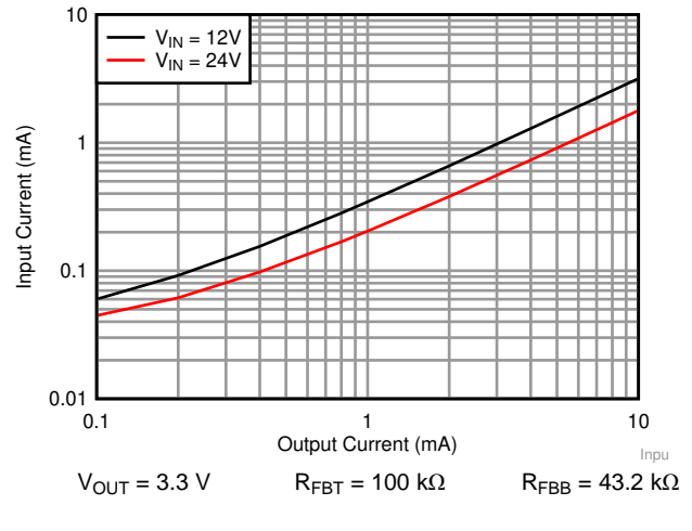
图 25. Input Supply Current versus Load Current
