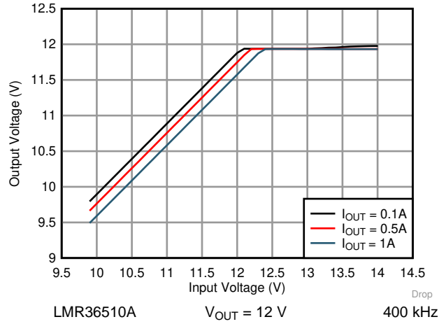
图 23. Dropout Characteristic
