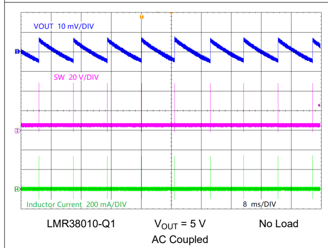
Figure 8-5. PFM Switching
