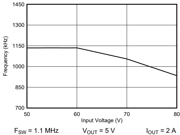
图 8-7. Typical Frequency Foldback at T ON_MIN
