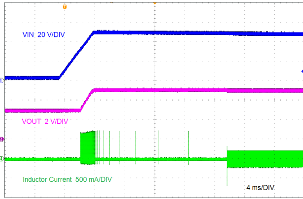
LMR38020F V_{OUT} = 5\text{ V} No Load Bias to 3 V
