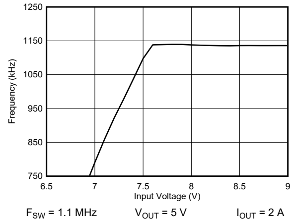
图 8-8. Typical Frequency Foldback at T OFF_MIN
