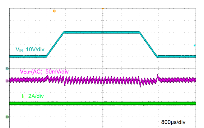
Figure 9-7. Line Transient
