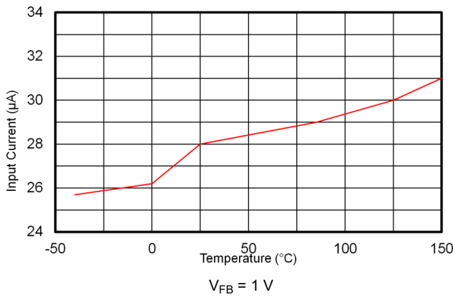
Figure 7-9. Non-Switching Input Supply Current
