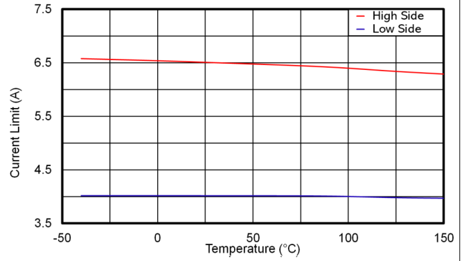
Figure 7-14. LMR51440 High Side and Low Side Current Limits
