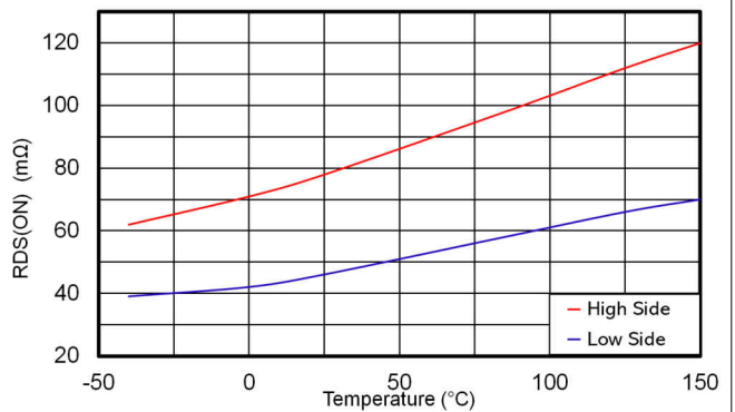
Figure 7-12. High Side and Low Side Switches R_{DS\_ON}
