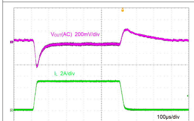
Figure 9-6. Load Transient
