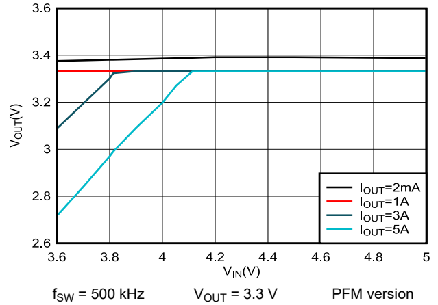
Figure 7-8. 3.3-V Dropout
