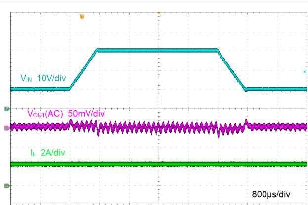
Figure 9-7. Line Transient
