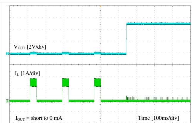
图 9-10. Short Recovery
