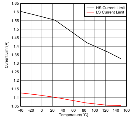
图 7-14. HS and LS Current Limit Versus Temperature
