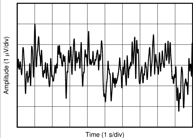
图 6-12. 0.1 Hz to 10 Hz Integrated Voltage Noise
