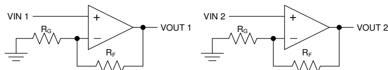
图 10-1. Schematic Representation for Figure 10-2
