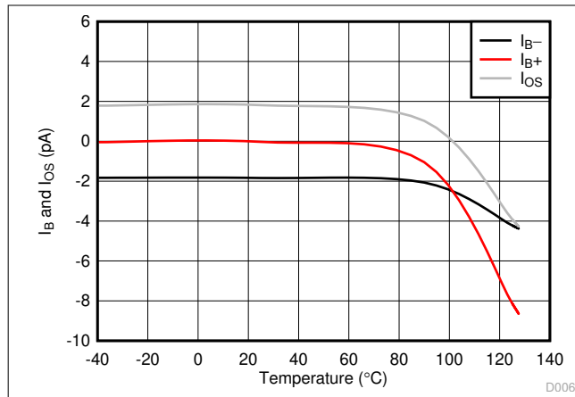
图 6-1. I_B and I_{OS} vs Temperature
