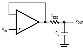
Figure 45. Isolation of C_{\text{L}} to Improve Stability
