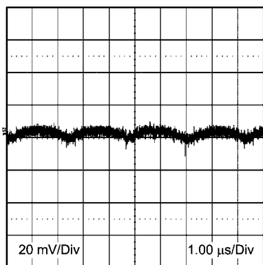
输出纹波 12V IN 3.3V O 2A 20mV/div 1μSec/div
