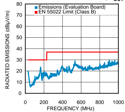
Radiated EMI of Evaluation Board, V_{OUT} = 12V
