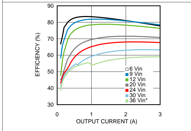
Figure 9. Efficiency 1.8-V Output at 25°C Ambient
