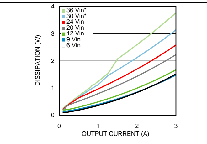
Figure 12. Dissipation 1.5-V Output at 25°C Ambient
