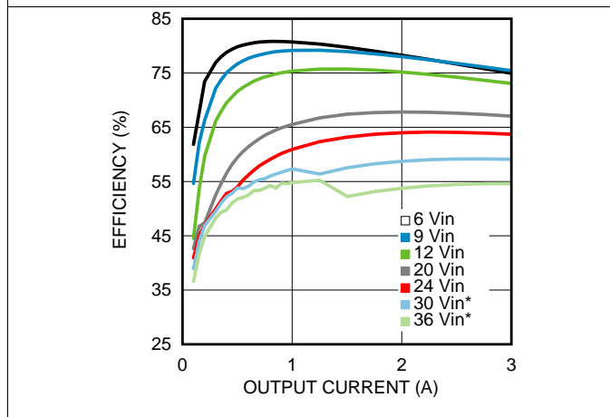
Figure 11. Efficiency 1.5-V Output at 25°C Ambient
