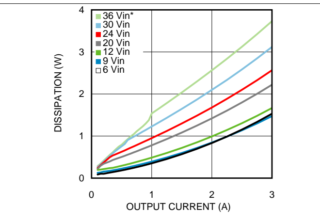
Figure 10. Dissipation 1.8-V Output at 25°C Ambient
