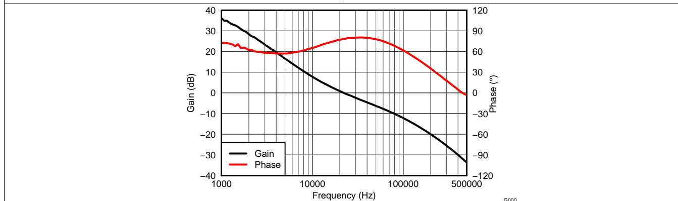
Figure 10. V_{OUT} = 1.8\text{ V} , I_{OUT} = 6\text{ A} , C_{OUT1} = 47\text{ }\mu\text{F} ceramic, C_{OUT2} = 100\text{ }\mu\text{F} POSCAP, f_{SW} = 1\text{ MHz}
