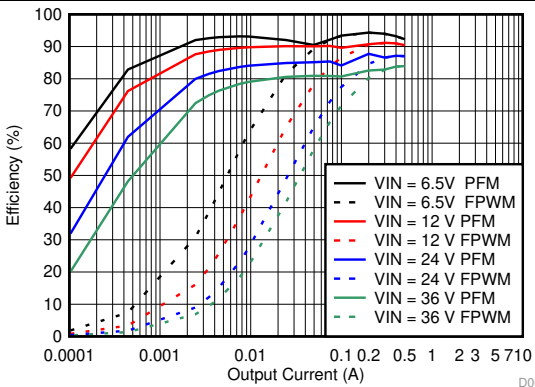
MODE = Low for Auto PFM Mode MODE = High for FPWM Mode 5-V Fixed Output
