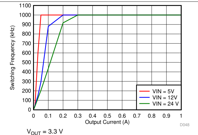
图 24. Auto PFM Mode Switching Frequency vs Output Current
