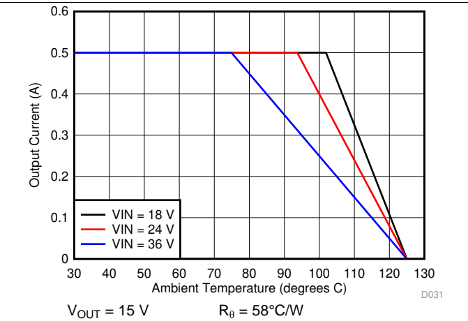
图 22. Ambient Temperature vs Output Current
